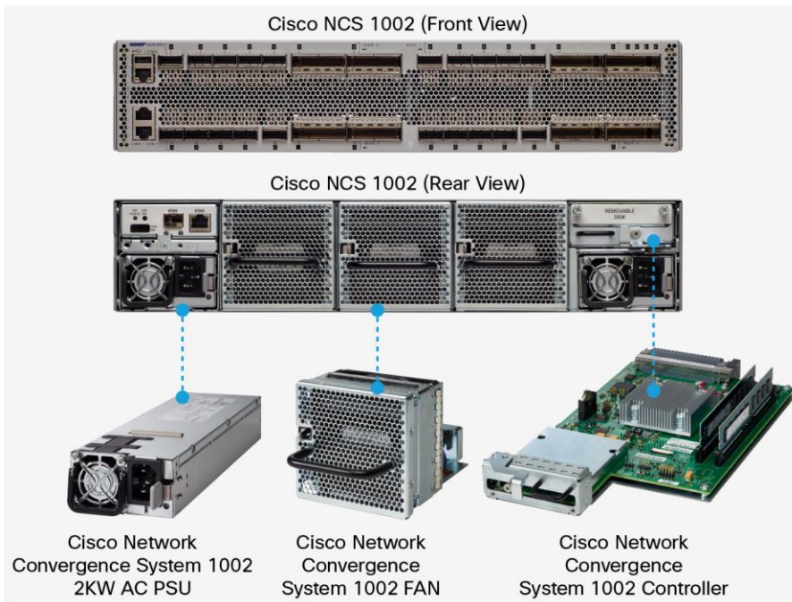
Figure 1. Cisco NCS 1002 Front and Rear Views, AC Power Supply Unit, Fan and Controller Card
